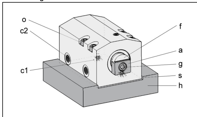
Figure 1: Components
