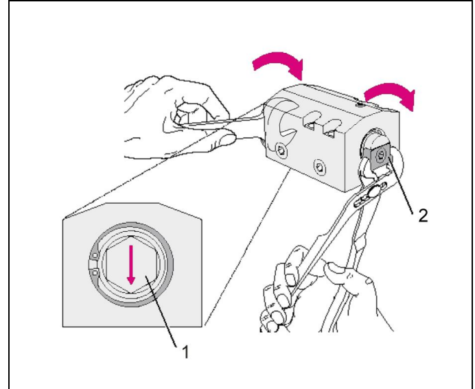
Figure 6: Schematic figure: Adjust clamping direction
