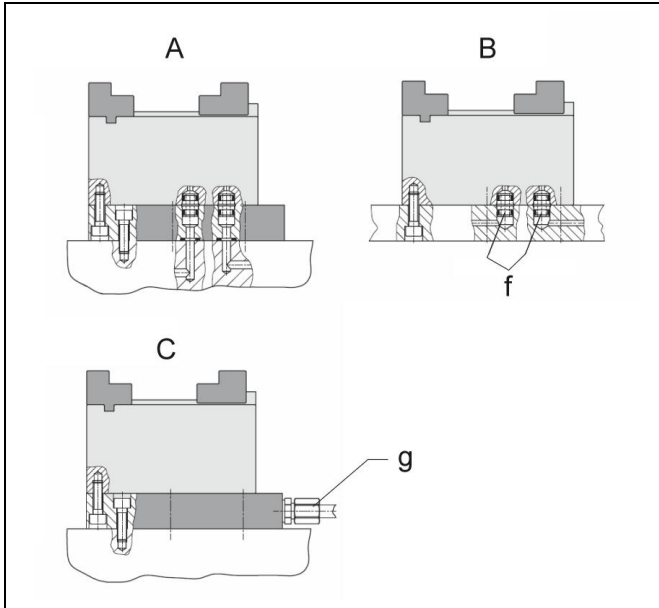
Figure 2: Mounting types
