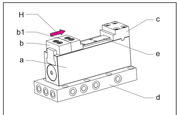
Figure 1: Components
